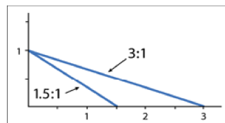
The slope is typically expressed as a ratio of the width of a structure's base to its height, or horizontal to vertical. This figure shows two examples of different slopes.
